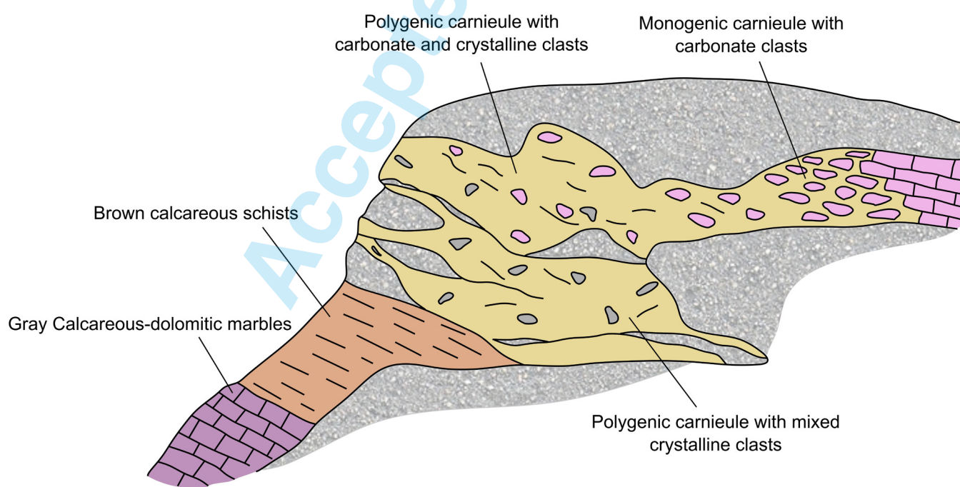
Fig. 44 - Geological simplified scheme of a typical carnieule outcrop of the meta-sedimentary cover of the Tambo nappe, redrawn after Metzeltin & Vezzoli (1977).
