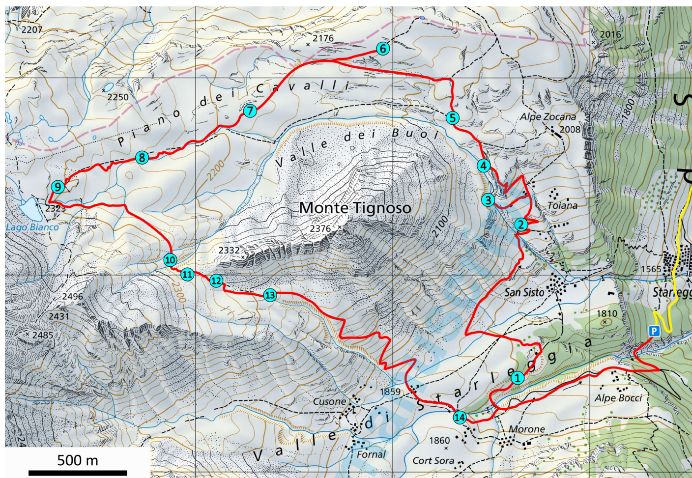
Fig. 2 - Field trip itinerary. Stops are marked by circles. Cartographic base: ©Federal Office of Topography swisstopo. Link to the online map: https://s.geo.admin.ch/0ovvg8cob5rt .
