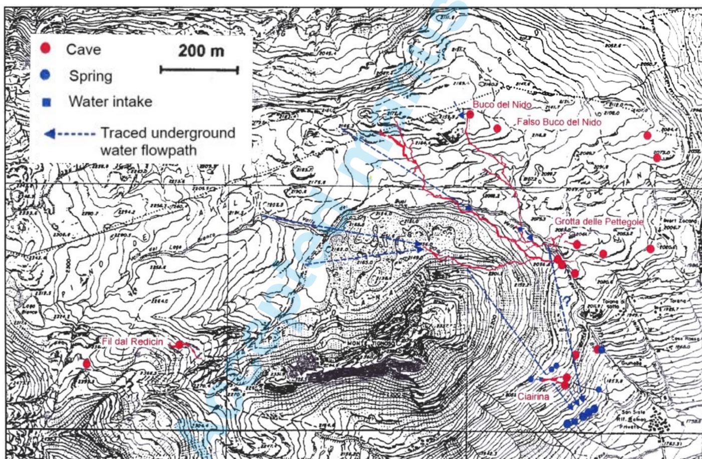
Fig. 33 - Plant map of caves at Pian dei Cavalli. Blue dashed arrows point to underground water pathways verified thanks to water tracing campaigns. Waters spring out NW of San Sisto (redrawn after Cella &amp; Torri, 1999).
