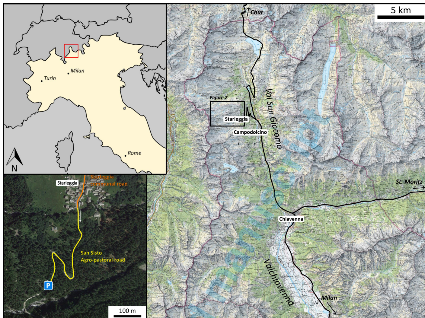
Fig. 1 - Location of the field trip area. Cartographic base: ©Federal Office of Topography swisstopo.
