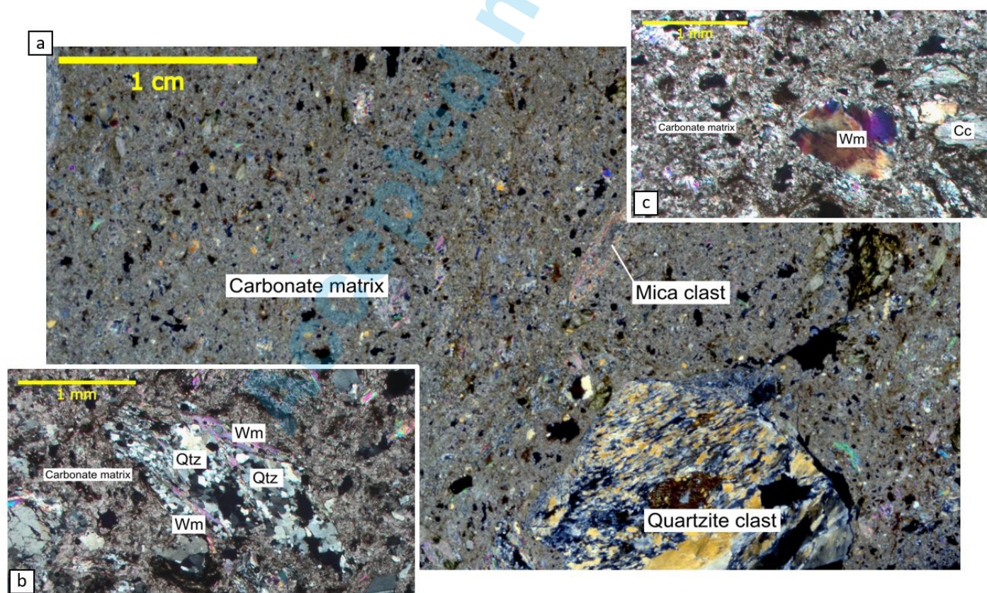
Fig. 14 - a) Thin section scan (crossed polars) of the Alpe Toiana tectonic breccias, with a cm-scale quartzite clast on the right; b) detail of a small clast composed by quartz grains and phengitic white mica (crossed polars); c) detail of a white mica mono-mineralic clast (crossed polars). Abbreviations: Cc = calcite; Qtz = quartz; Wm = white mica.
