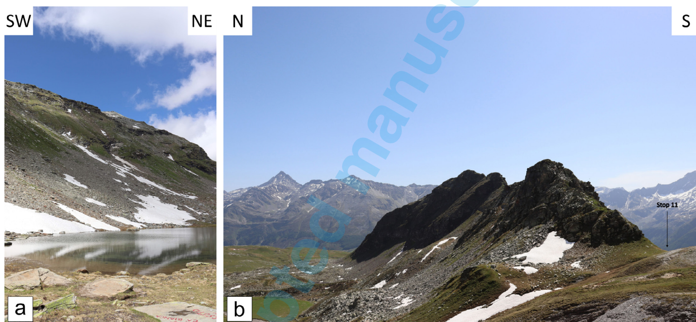
Fig. 38 - a) The Lago Bianco area and the eastern flank of Monte Bardan, made up of paragneisses from the Tambo nappe; b) Monte Tignoso area located south of Pian dei Cavalli. Location of Stop 11 is indicated.
