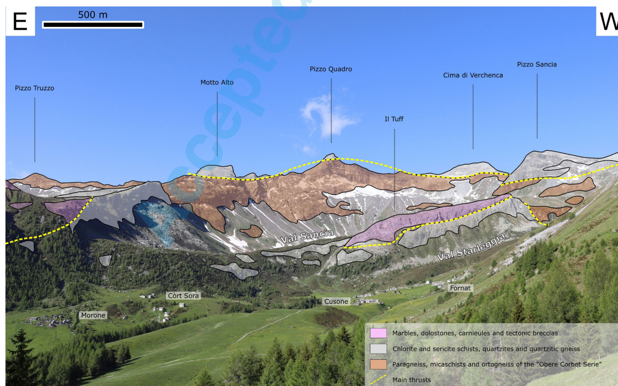
Fig. 52 - Panoramic view of Val Sancia, as seen from the southern slope of Monte Tignoso.
