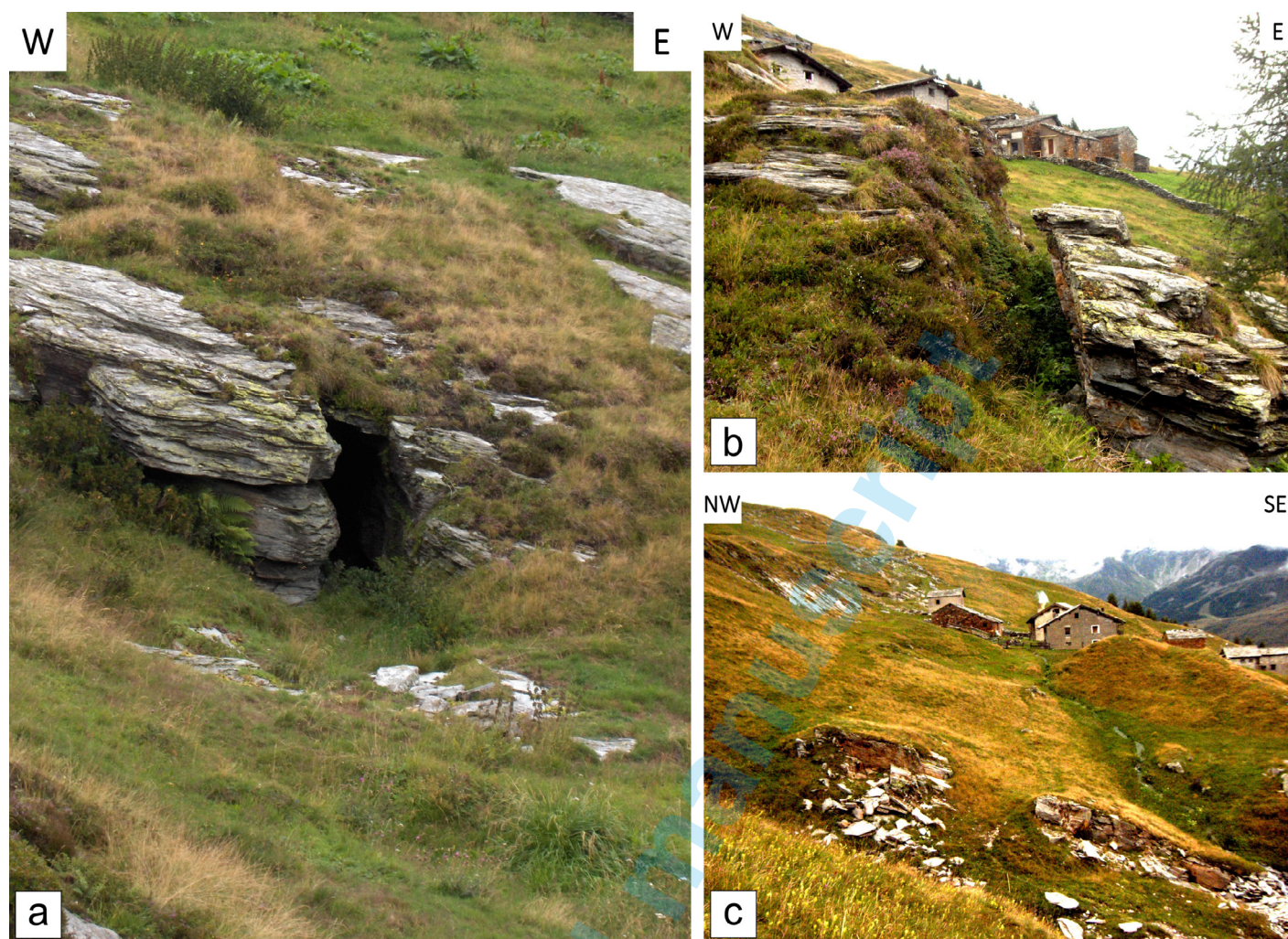
Fig. 11 - a) and b) Meter-sized open fractures on the slope south of Alpe Toiana; c) trenches at Alpe Toiana.
