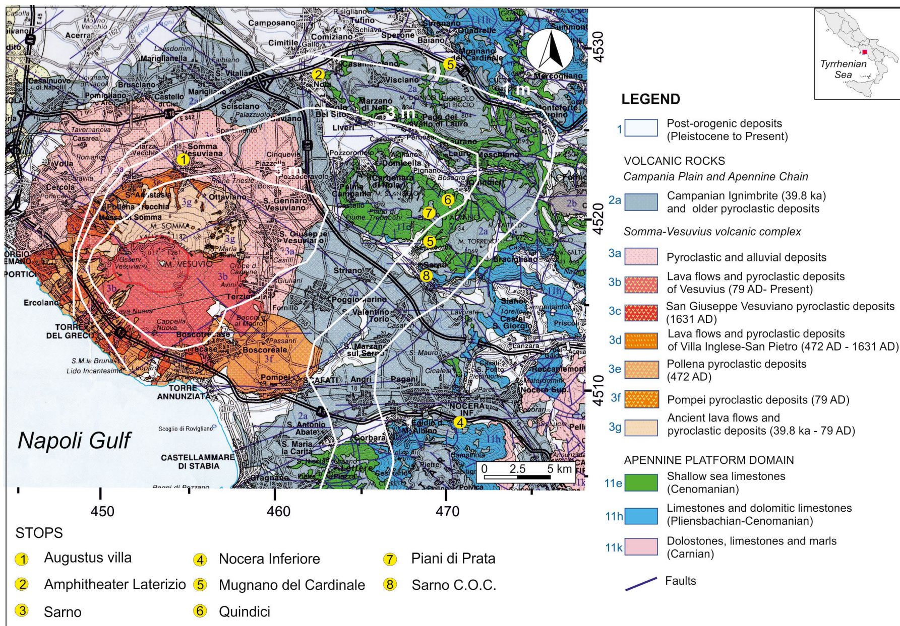
Fig. 2 - Location of the proposed on-land stops on the 1:250.000 Geological Map of Campania modified after Ciarcia and Vitale (2018). The white contours, redrawn from Lirer et al. (2001), are the isopaches summing the thicknesses of all the pyroclastic fall deposits emplaced by Somma-Vesuvius in the last 10 kysr.
