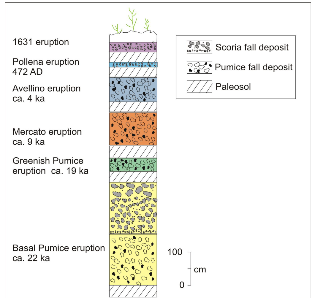
Fig. 26 – Composed type section of the Somma-Vesuvius pyroclastic fall deposits at Piani di Prata. Map of the area in Fig. 2.
