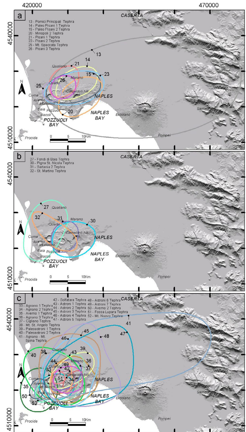
Fig. 3 - Distribution of the pyroclastic fallout deposits of the past 15 kyrs at the Campi Flegrei caldera (from Orsi et al., 2004). a, b and c: fallout beds thicker than 10 cm of the I, II and III epoch, respectively.
