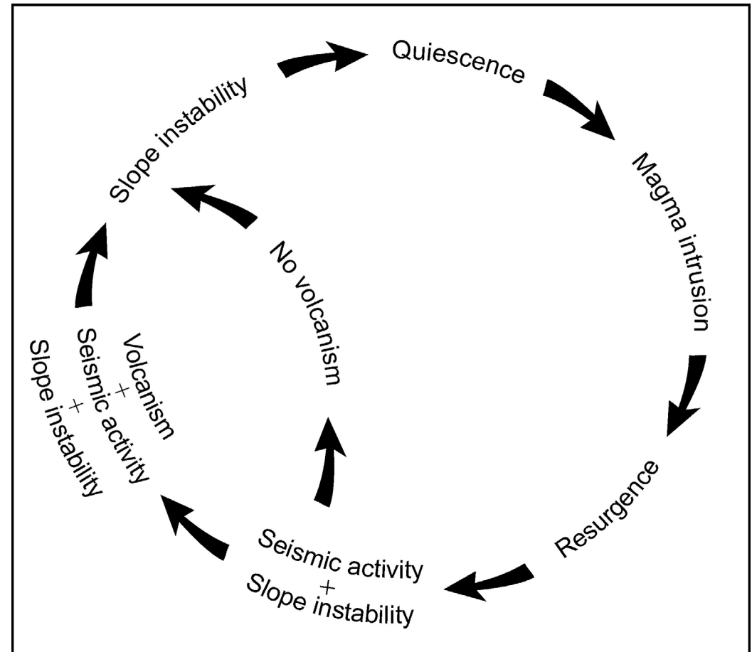
Fig. 6 - Cyclical behavior of phenomena occurring at Ischia at variable time intervals. Starting from a quiescence period, a new magma intrusion triggers resurgence, and therefore deformation, which is accompanied by seismicity and slope instability. Renewal of volcanism may or may not occur, being accompanied and followed by seismic activity and slope instability. Slope instability could last many centuries, during the following quiescence period (after de Vita et al., 2006).
