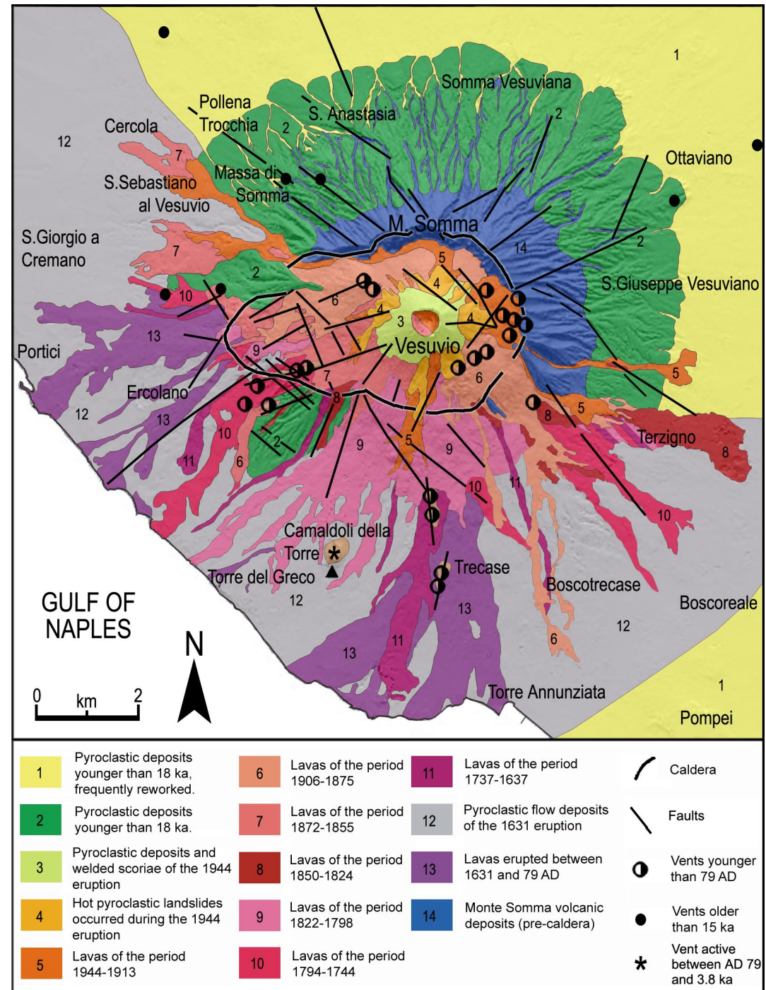
Fig. 4 - Somma-Vesuvius geological sketch map (after Orsi et al., 2003). Structural lineaments after Ventura and Vilardo, 1999).
