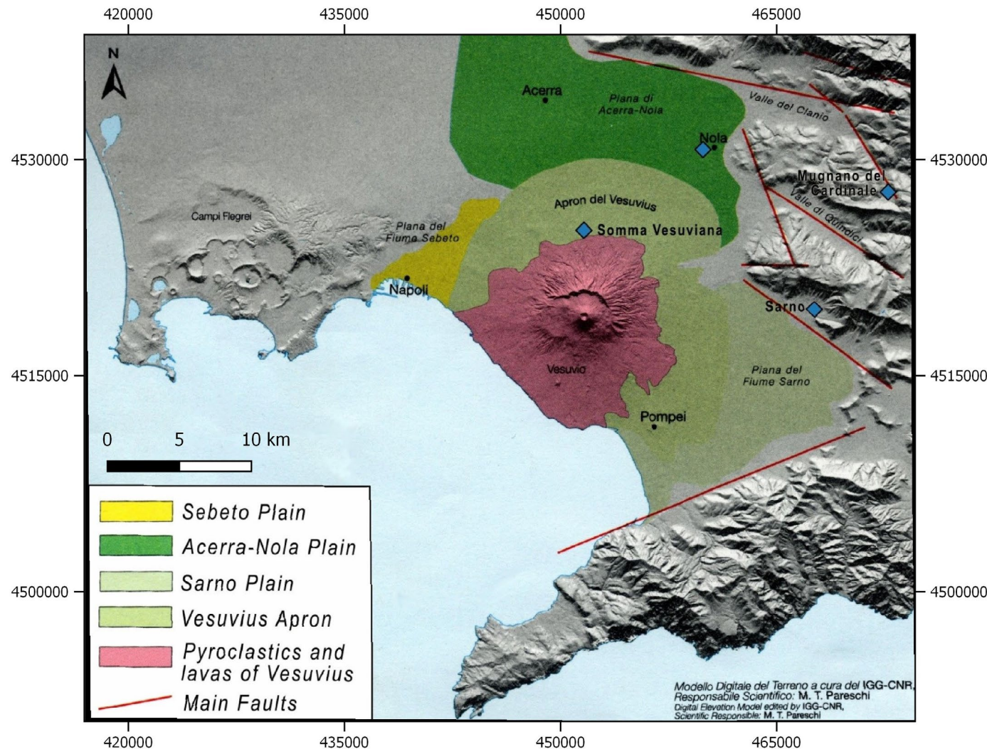
Fig. 10 - Sketch map of the Vesuvius edifice and the surrounding plain and Apennines. The Villa di Augusto is located in the northern sector of the Vesuvius Apron, the Nola Amphitheater in the Nola Plain at the mouth of the Quindici Valley-Vallo di Lauro.
